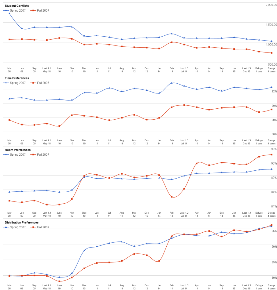
Fig. 7 Value of the four optimization criteria, compared using the latest solver.
