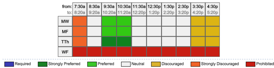
Fig. 2 Example 2 x 50 time pattern
