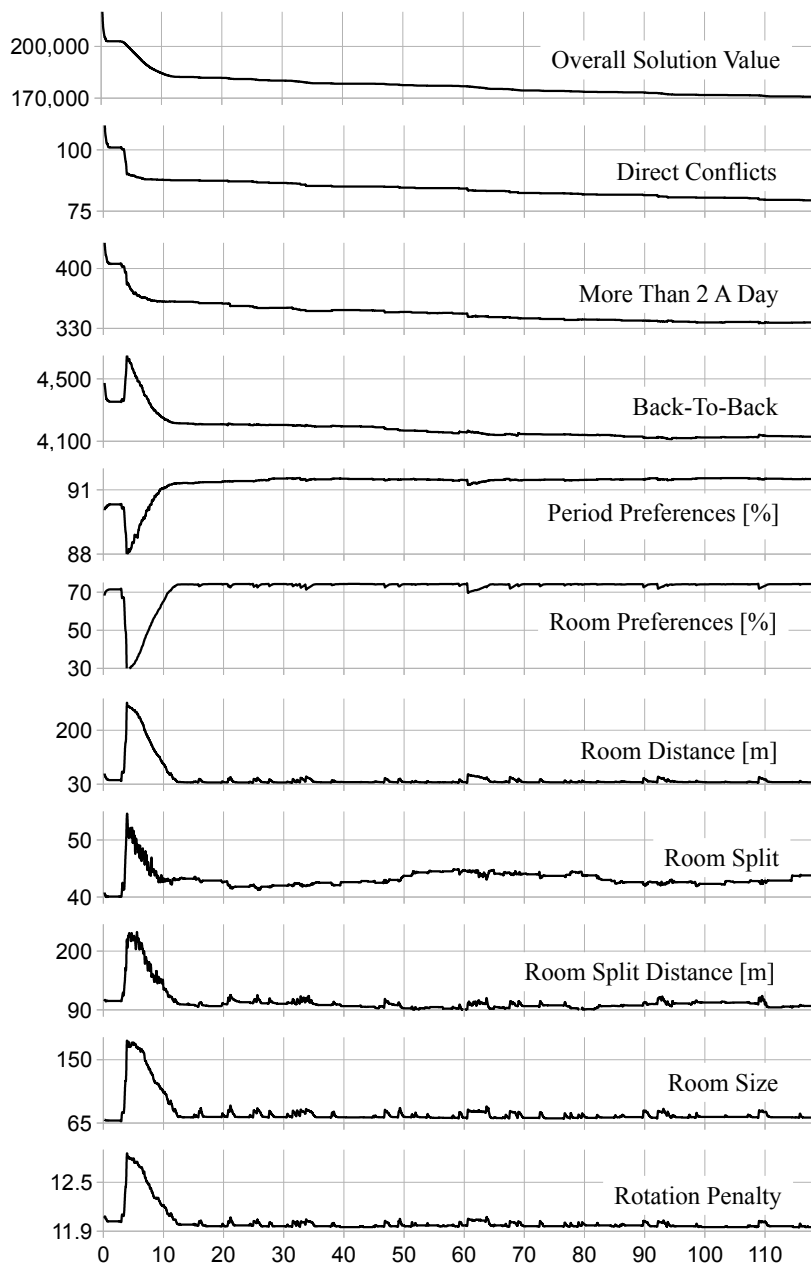
Fig. 5 Progression of the best computed solution during the search. Each chart represents one objective, the horizontal axe represents time in minutes. Average results of 10 independent runs on the Fall 2012 problem using production configuration are presented.
